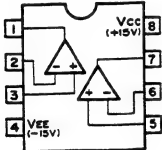
uPC4556C (NEC) OPERATIONAL AMPLIFIER (WIDE BAND, DECOMPENSATED) — TOP VIEW —
